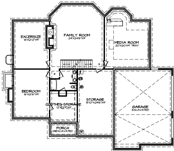
FOUNDATION PLAN A-2
