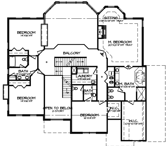
SECOND FLOOR PLAN A-4
