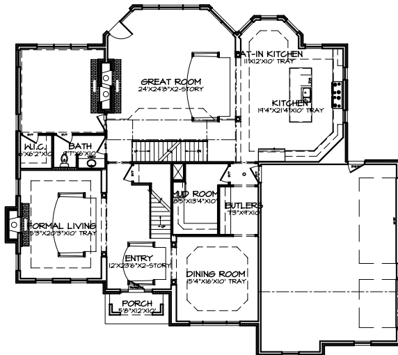
FIRST FLOOR PLAN A-3
